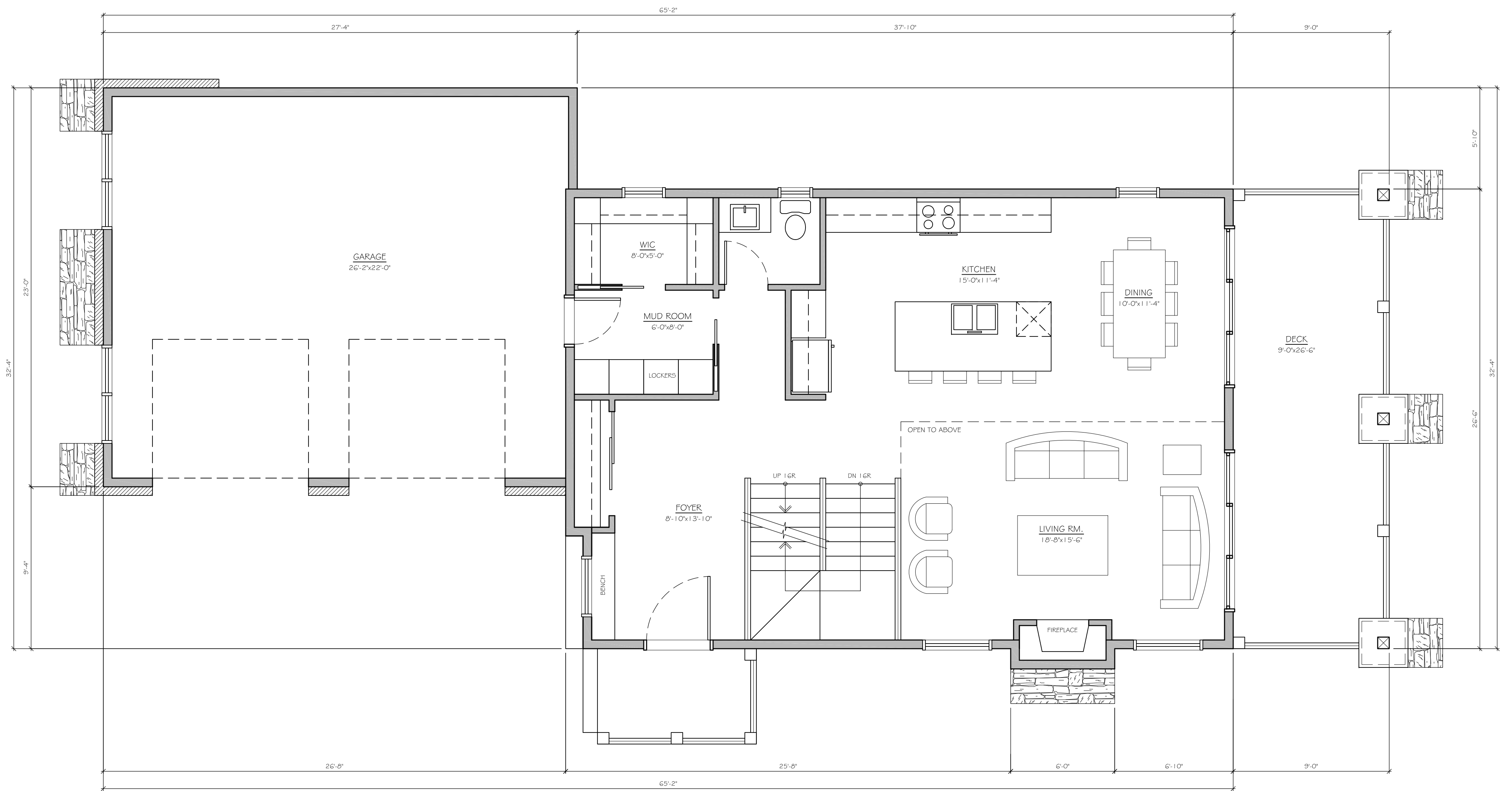
1 MAIN FLOOR PLAN AP 1/4" = 1'-0" 1020 ft. 2 610 ft. 2 GARAGE
